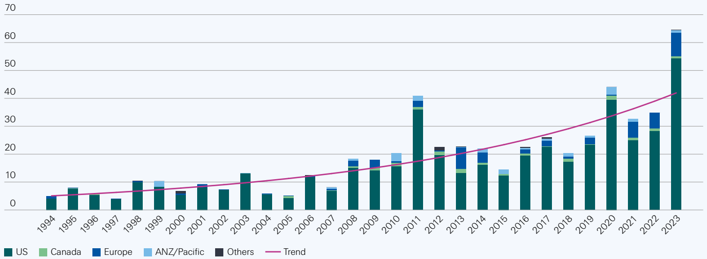
Figure 10 Annual insured losses from SCS per region, (USD bn, 2023 prices), and global trend
