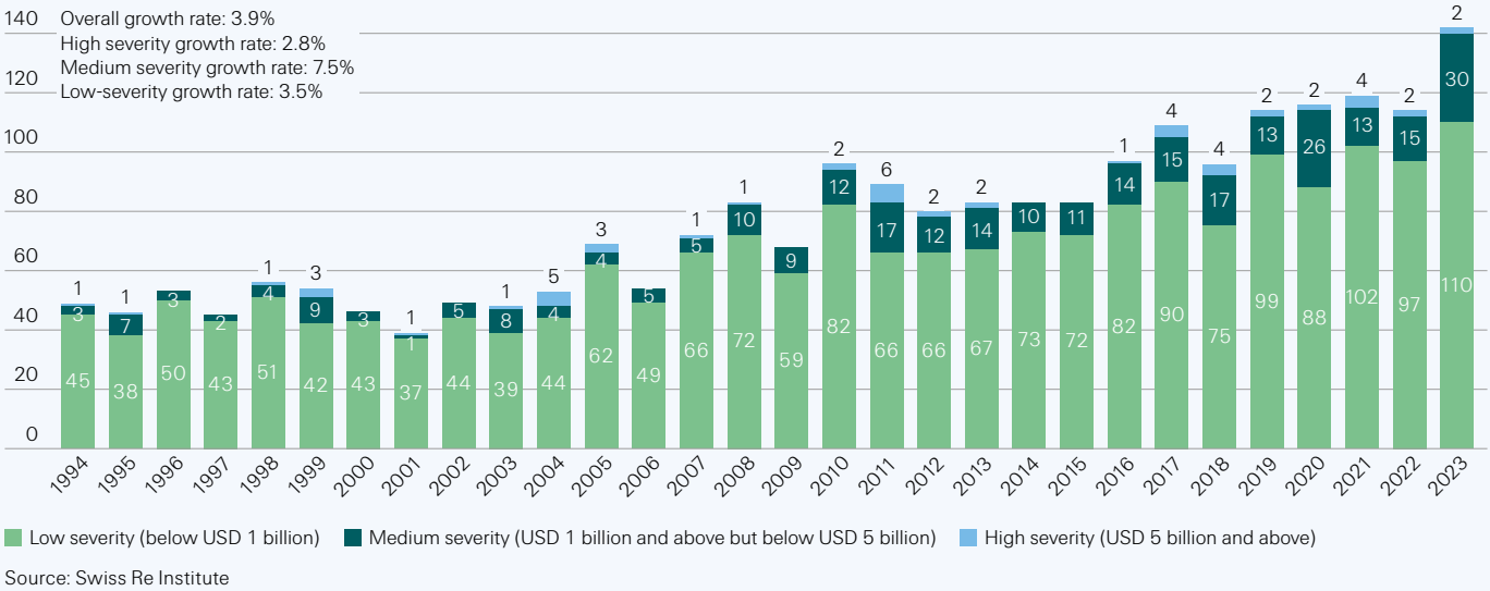
Figure 5 Number of natural catastrophes by classes of severity, 1994–2023
